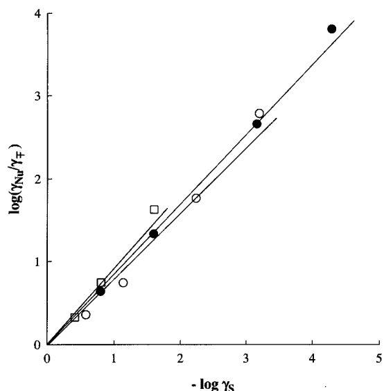
Figure 3. Relationships between \log(\gamma_{\text{Nuc}}/\gamma_{\pm}) and \log \gamma_s for reactions with 2-hydroxybenzaldehyde ion (BAO-OH) in \text{H}_2\text{O} -MeCN. Symbols as in Fig. 1
