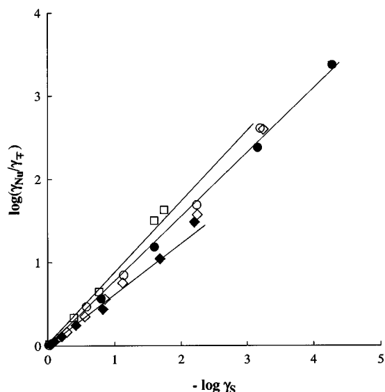
Figure 1. Relationships between \log(\gamma_{\text{Nu}}/\gamma_{\text{T}}) and \log \gamma_{\text{S}} for reactions with \text{OH}^- in \text{H}_2\text{O} -MeCN: (●) (\text{PhO})_2\text{POOAr} ; (○) \text{Ph}_2\text{POOAr} ; (◇) \text{Ph}_2\text{POSPH} ; (◆) \text{Ph}_2\text{POSEt} ; (□) \text{Ph}(\text{Et})\text{POOAr}
