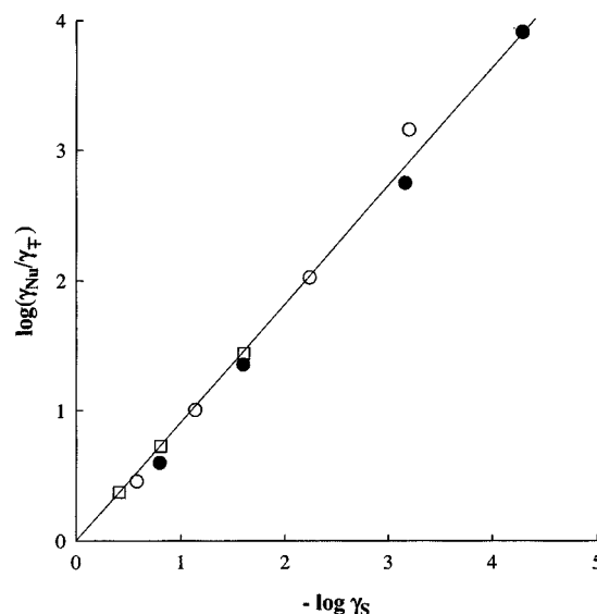
Figure 2. Relationships between \log(\gamma_{\text{Nu}}/\gamma_{\text{T}}) and \log \gamma_{\text{S}} for reactions with 2,3-butanedionemonooximate ion (BDO) in \text{H}_2\text{O} -MeCN. Symbols as in Fig. 1
